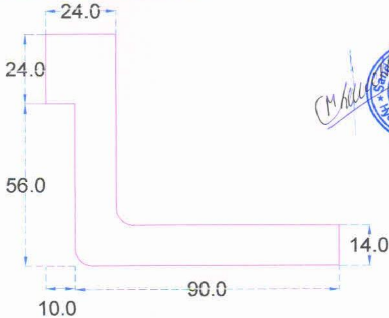
DAM GATE RUBBER SEAL (Z-TYPE)
