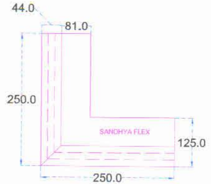
DETAILS OF MOULDED CORNER SEAL
