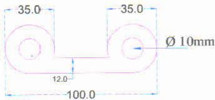
SECTIONAL DETAILS OF DOUBLE HOLLOW BULB DAM GATE SEAL
