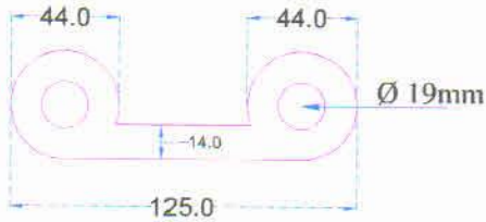
SECTIONAL DETAILS OF DOUBLE HOLLOW BULB DAM GATE SEAL
