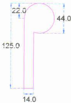
SECTIONAL DETAILS OF MUSICAL NOTE DAM GATE SEAL
