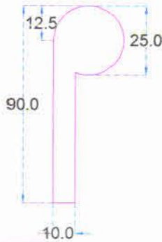
SECTIONAL DETAILS OF MUSICAL NOTE DAM GATE SEAL
